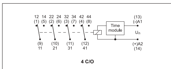
Connection diagram
